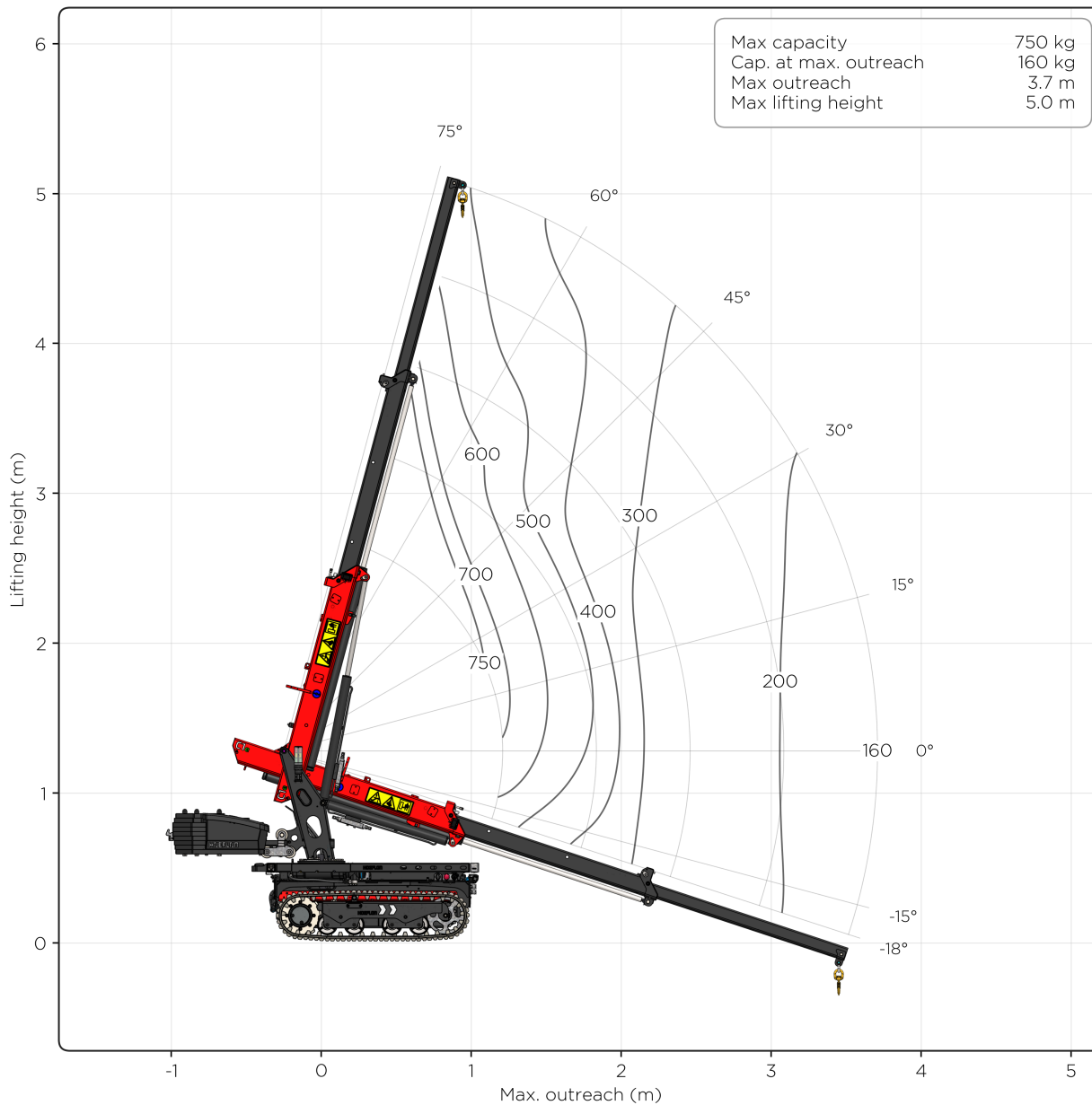
C1 Loadchart - main boom
