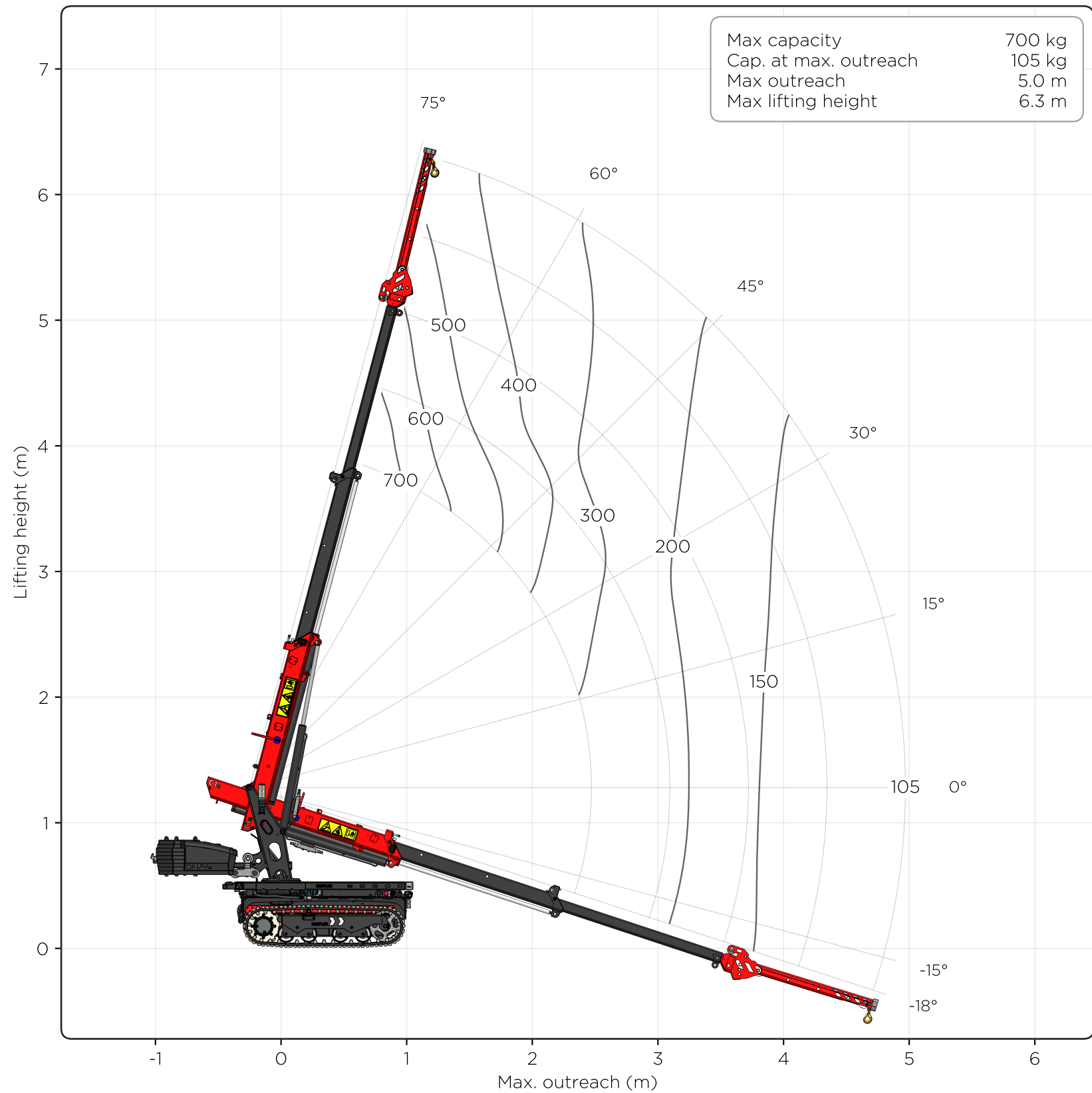
C1 Loadchart - with searcher hook
